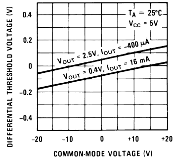
Common-Mode Voltage Sensitivity
