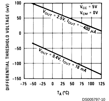
Temperature Sensitivity
