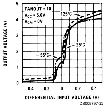
Transfer Function
