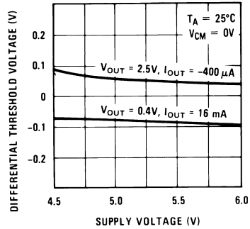
Supply Voltage Sensitivity
