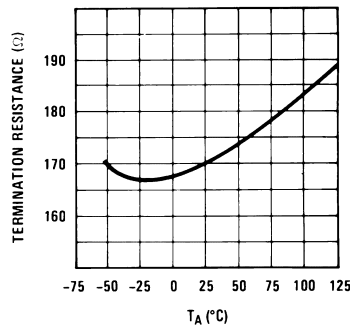
Termination Resistance
