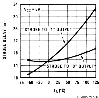
Strobe Delays
