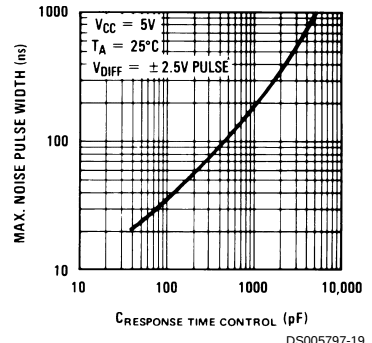
Noise Rejection
