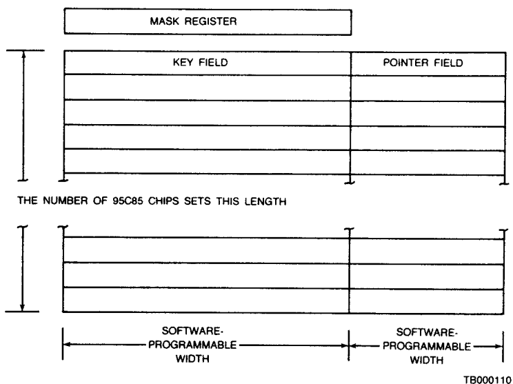
Figure 2. Am95C85 CADM Programmer's Model
