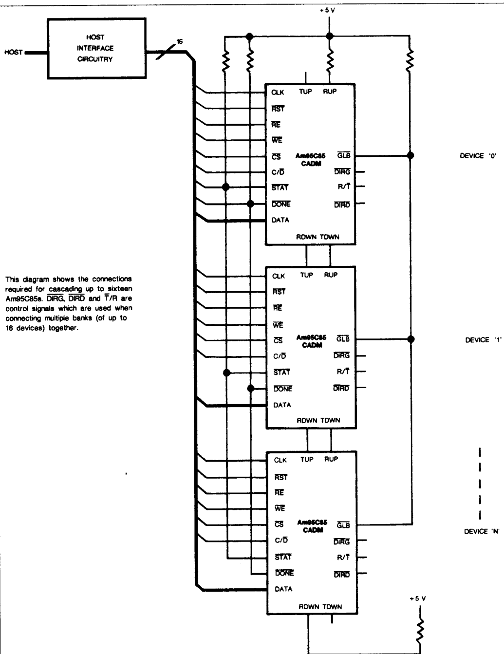
Figure 3. Am95C85 Cascade Circuit
