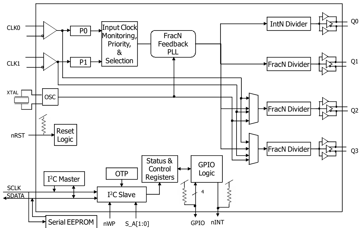
Figure 1. 8T49N241 Block Diagram
