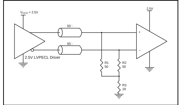
Figure 13C. 2.5V LVPECL Driver Termination Example
