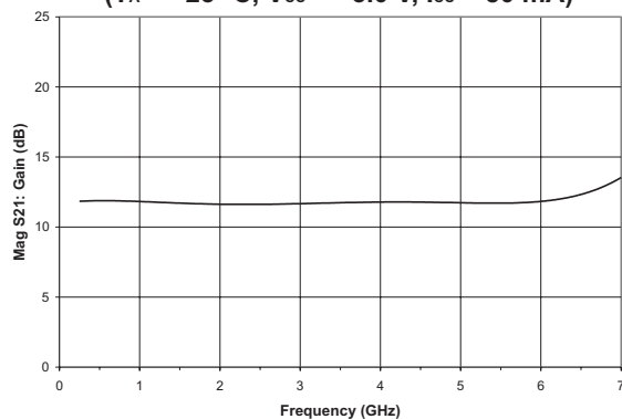
Figure 4: Gain vs. Frequency De-embedded 50 \Omega S-parameter (T A = +25 °C, V CC = +5.0 V, I CC = 80 mA)
