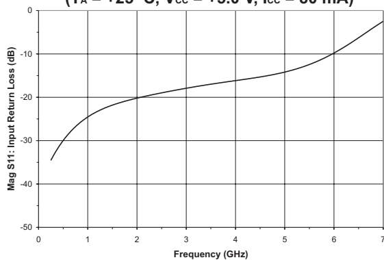
Figure 6: Input Return Loss vs. Frequency De-embedded 50 \Omega S-parameter (T A = +25 °C, V CC = +5.0 V, I CC = 80 mA)
