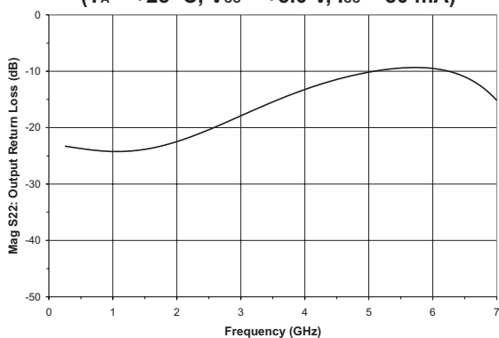
Figure 7: Output Return Loss vs. Frequency De-embedded 50 \Omega S-parameter (T A = +25 °C, V CC = +5.0 V, I CC = 80 mA)
