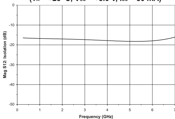
Figure 5: Isolation vs. Frequency De-embedded 50 \Omega S-parameter (T A = +25 °C, V CC = +5.0 V, I CC = 80 mA)
