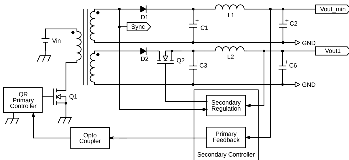
Figure 39. Regulation Principle Schematic
