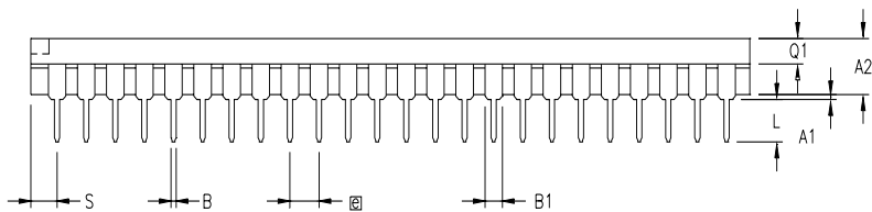
Figure 29.48-Pin DIP
