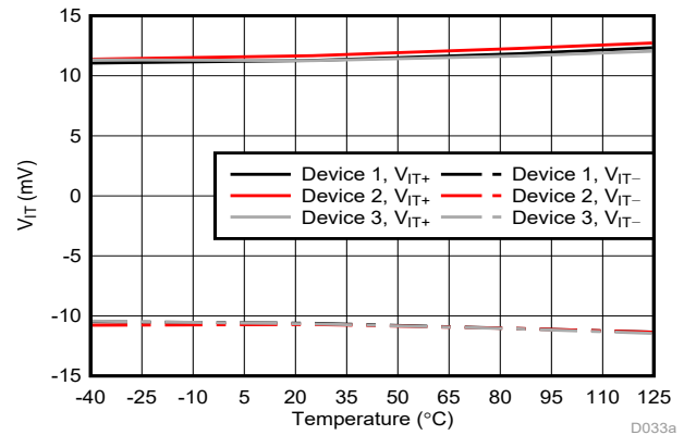
Figure 6-6. Trip Threshold vs Temperature
