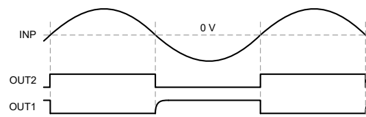
Figure 6-2. Functional Timing Diagram
