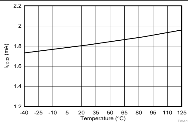
Figure 6-18. High-Side Supply Current vs Temperature
