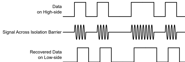
Figure 7-2. OOK-Based Modulation Scheme
