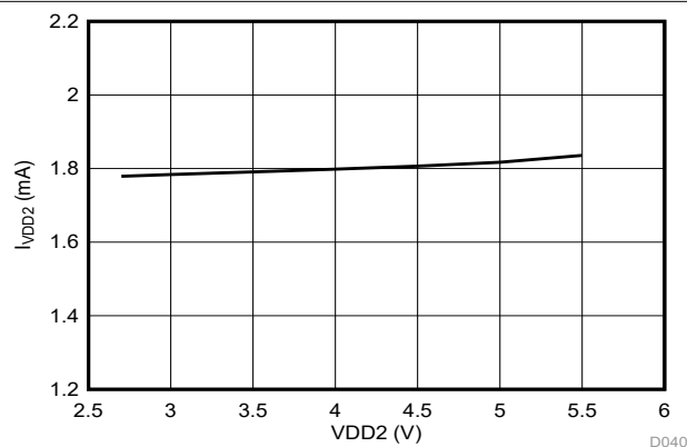
Figure 6-17. High-Side Supply Current vs Supply Voltage
