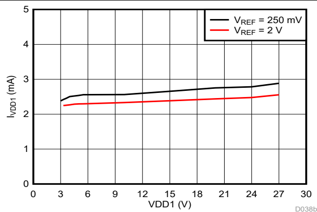
Figure 6-17. High-Side Supply Current vs Supply Voltage
