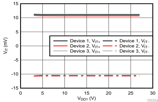
Figure 6-5. Trip Threshold vs Supply Voltage
