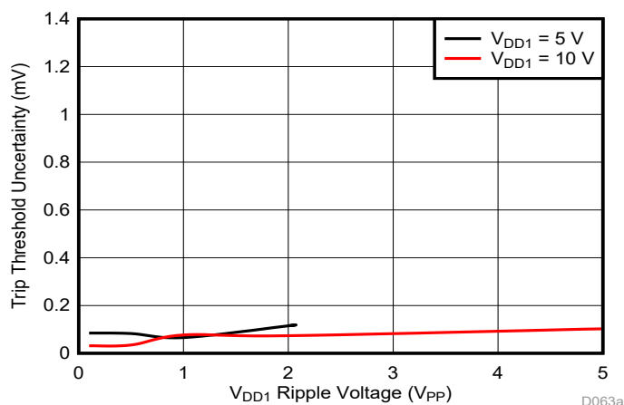
Figure 8-5. Trip Threshold Sensitivity to VDD1 Ripple Voltage (f RIPL = 10 kHz)
