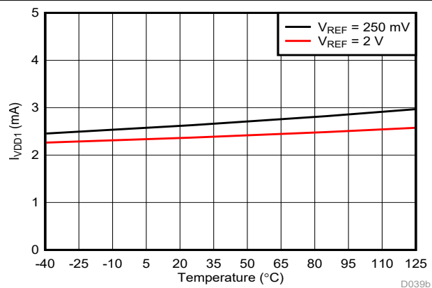
Figure 6-18. High-Side Supply Current vs Temperature
