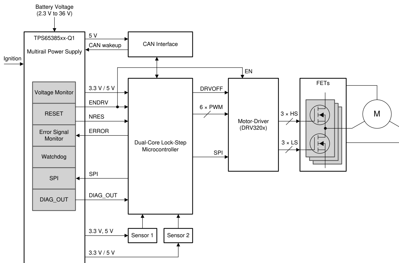
Figure 1-1. Typical Application Diagram
