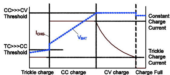
a) Without input current limit
