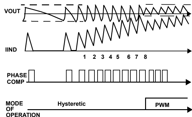
FIGURE 4. HYSTERETIC -- CCM TRANSITION
