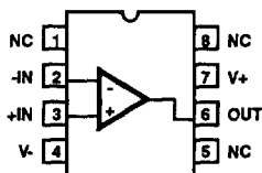
HFA1100/883 (CERDIP) TOP VIEW
