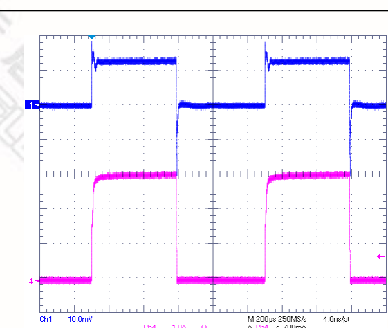
VIN=1.2V, VCNTL=5V, VOUT=0.6V @ 3A Sinking
