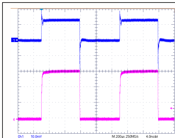
VIN=1.5V, VCNTL=5V, VOUT=0.75V @ 3A Sinking
