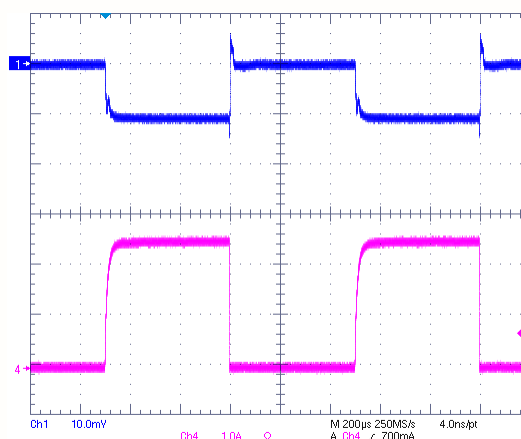
VIN=2.5V, VCNTL=5V, VOUT=1.25V @ 2.5A Sourcing
