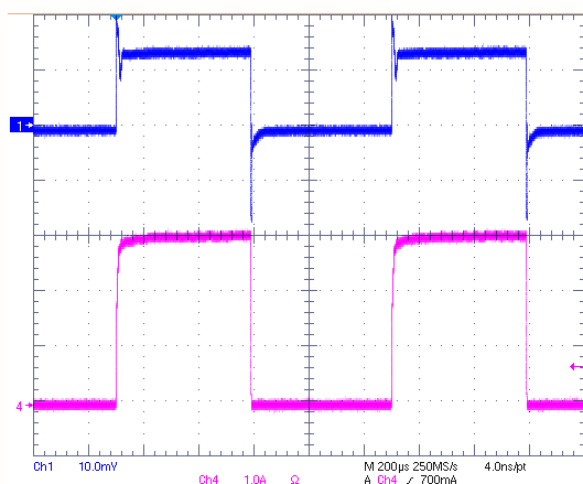
VIN=2.5V, VCNTL=3.3V, VOUT=1.25V @ 3A Sinking
