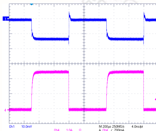
VIN=2.5V, VCNTL=3.3V, VOUT=1.25V @ 2.5A Sourcing
