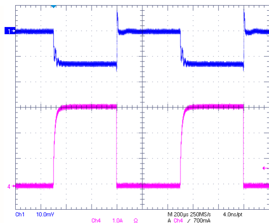
VIN=1.2V, VCNTL=5V, VOUT=0.6V @ 3A Sourcing
