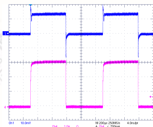
VIN=2.5V, VCNTL=5V, VOUT=1.25V @ 3A Sinking
