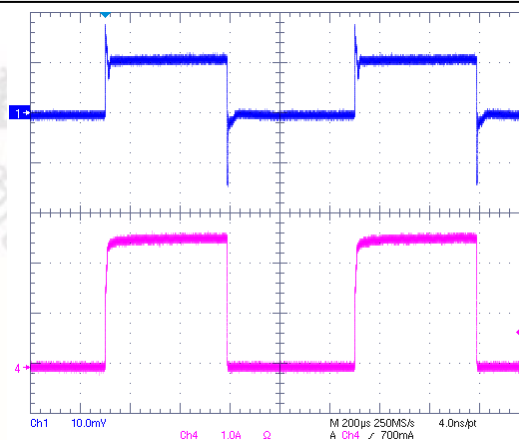
VIN=1.8V, VCNTL=3.3V, VOUT=0.9V @ 2.5A Sinking
