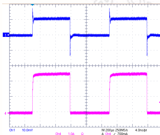
VIN=1.8V, VCNTL=5V, VOUT=0.9V @ 2.5A Sinking
