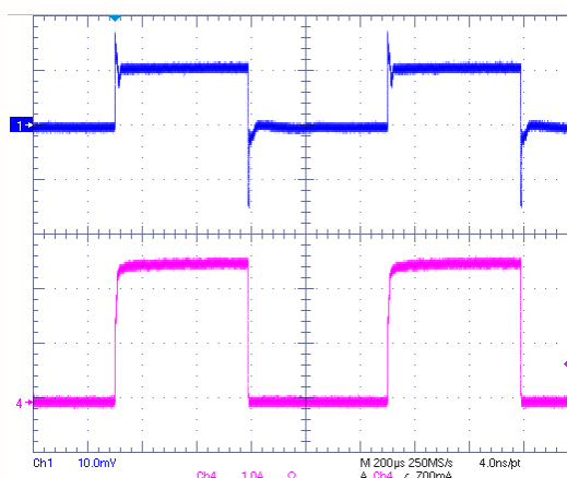
VIN=1.5V, VCNTL=3.3V, VOUT=0.75V @ 2.5A Sinking
