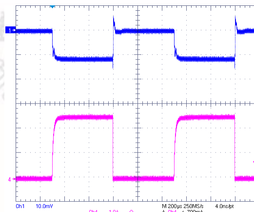
VIN=1.8V, VCNTL=3.3V, VOUT=0.9V @ 2.5A Sourcing
