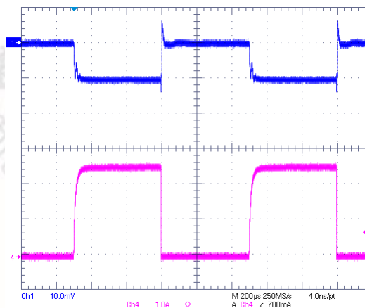
VIN=1.2V, VCNTL=5V, VOUT=0.6V @ 2.5A Sourcing
