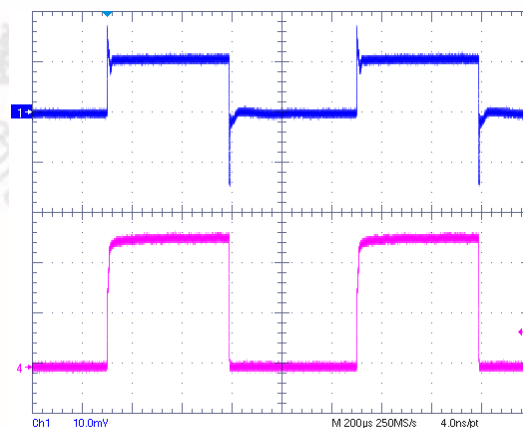
VIN=1.5V, VCNTL=5V, VOUT=0.75V @ 2.5A Sinking
