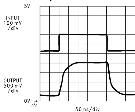
LM7131 Cable Driver A_V = +10 @ +3V
