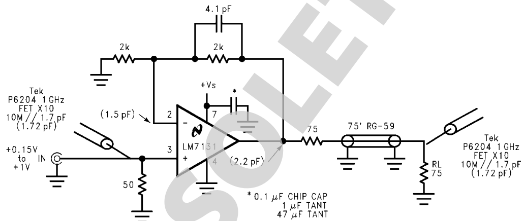
FIGURE 3. Cable Driver 5' RG-59
