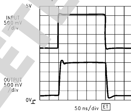
LM7131 Cable Driver A_V = +1 @ +5V
