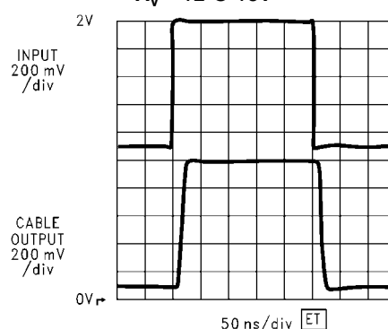
LM7131 Driving 5' RG-59 A_V = +2 @ +5V
