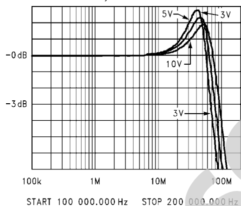
LM7131 Bode Plot @ 3V, 5V and 10V
