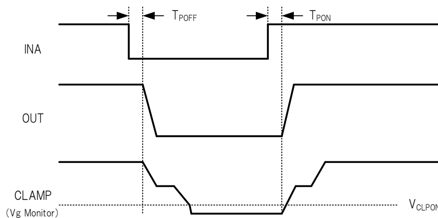
Timing chart of Miller clamp function
