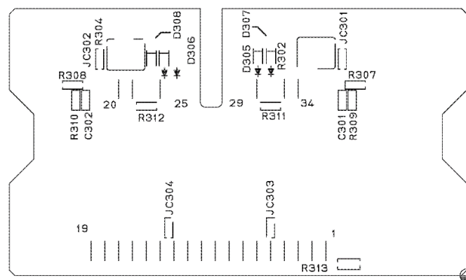
Solder side
