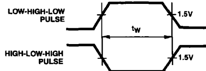
FIGURE 3. PULSE WIDTH
