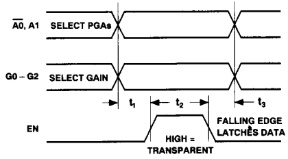
Timing Diagram 1. AD75062
