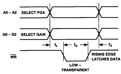
Timing Diagram 2. AD75068
