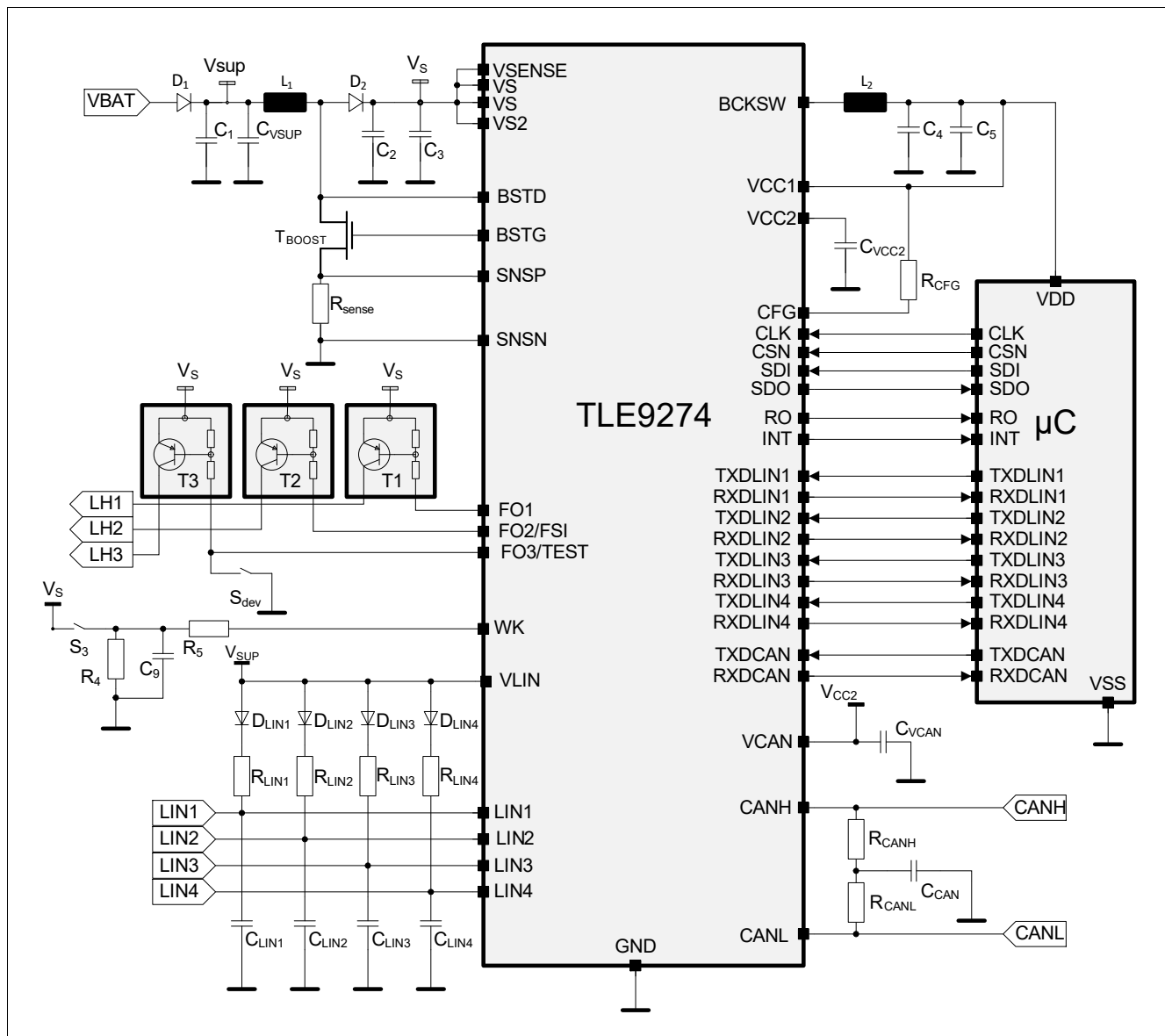
Figure 51 Application diagram
