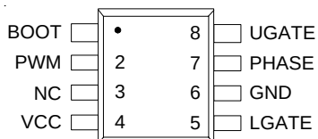
SOP-8
