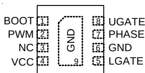
WDFN-8EL 3x3
