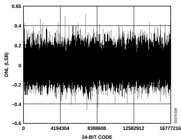
Figure 20. 24-Bit DNL
