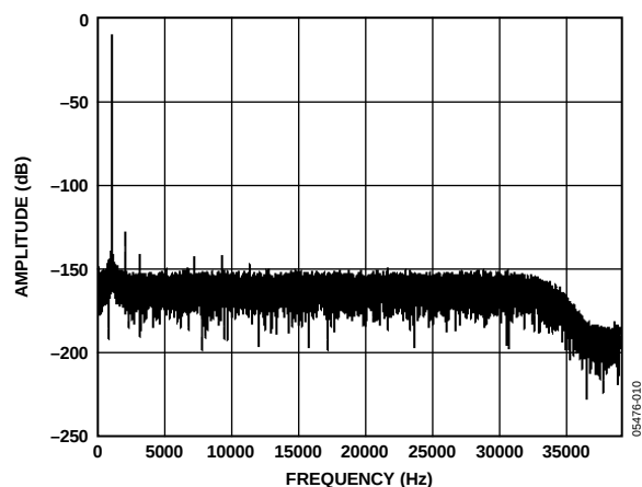
Figure 10. Low Power FFT, 1 kHz, -0.6 dB Input Tone, 256 \times Decimation
