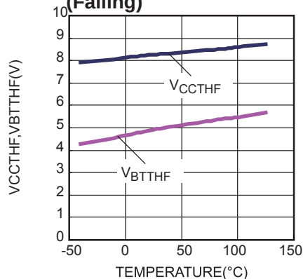
Undervoltage Lockout Threshold (Falling)
