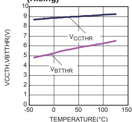
Undervoltage Lockout Threshold (Rising)
