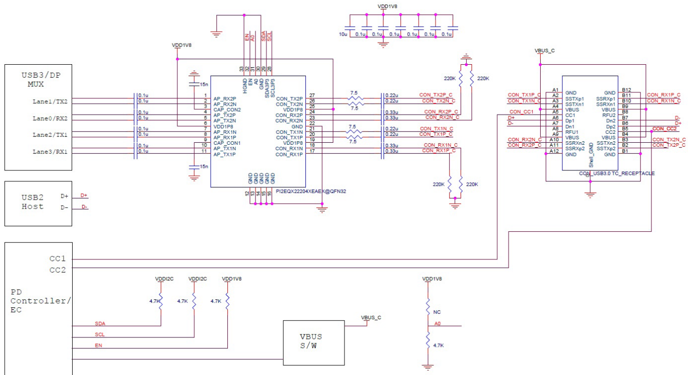
Figure 6-1 PI2EQX22024 Reference Schematic
