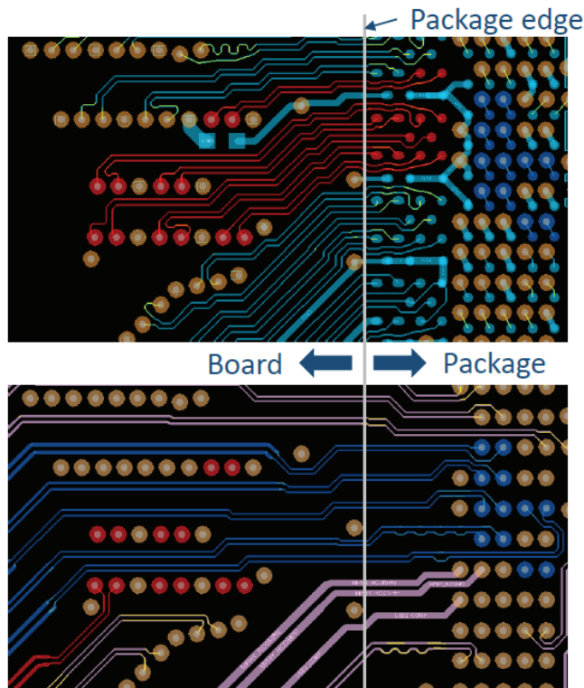
Figure 6-12 Breakout Tx and Rx I/O on Different PCB Layers
