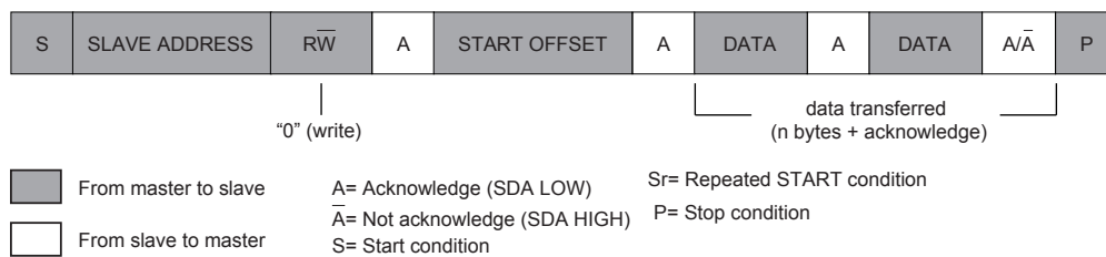
Figure 4-6 Indexed Write Protocol
