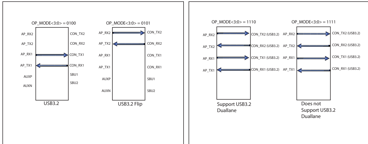
Figure 2-1 The Channel Configuration Against the OP_MODE<3:0>
