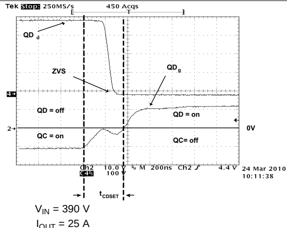
Figure 62. Full-Bridge Gate Drives and Switch Nodes (QD a QD d )
