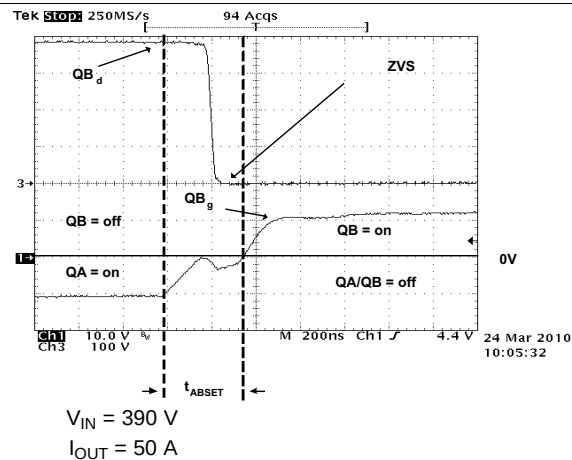
Figure 63. Full-Bridge Gate Drives and Switch Nodes (QB q QB d )
