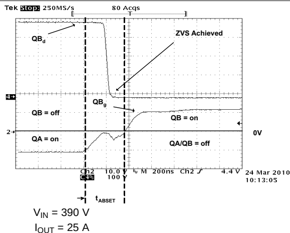
Figure 61. Full-Bridge Gate Drives and Switch Nodes (QB q QB d )
