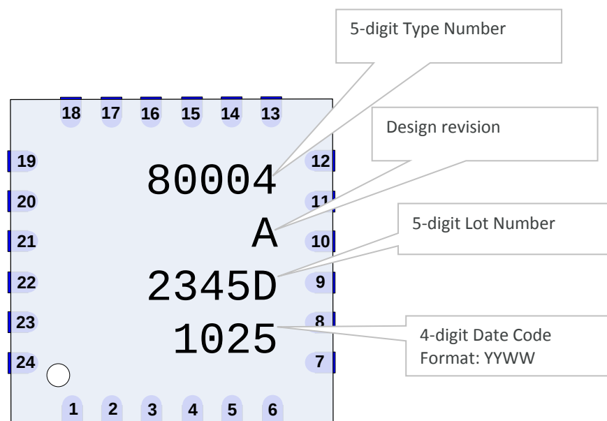
Figure 12: Package marking, example for MLX80004 in QFN4x4 24L
