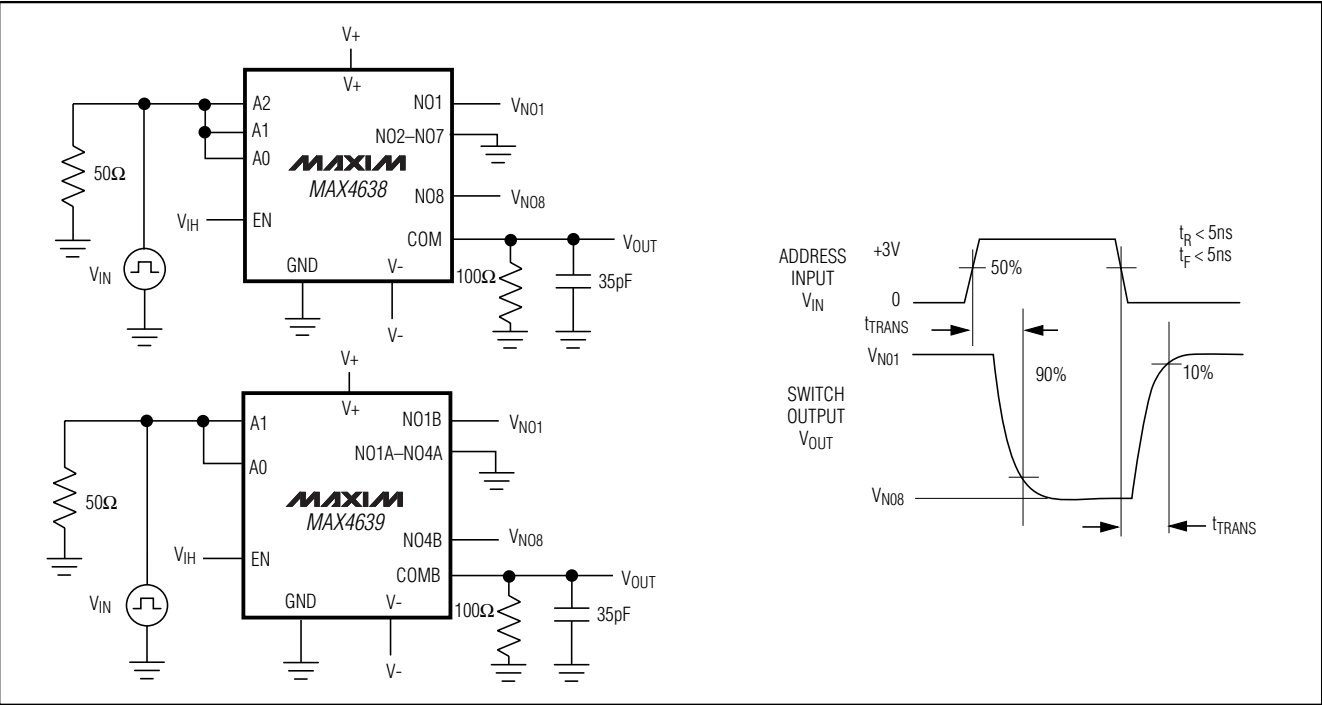
Figure 2. Transition Time
