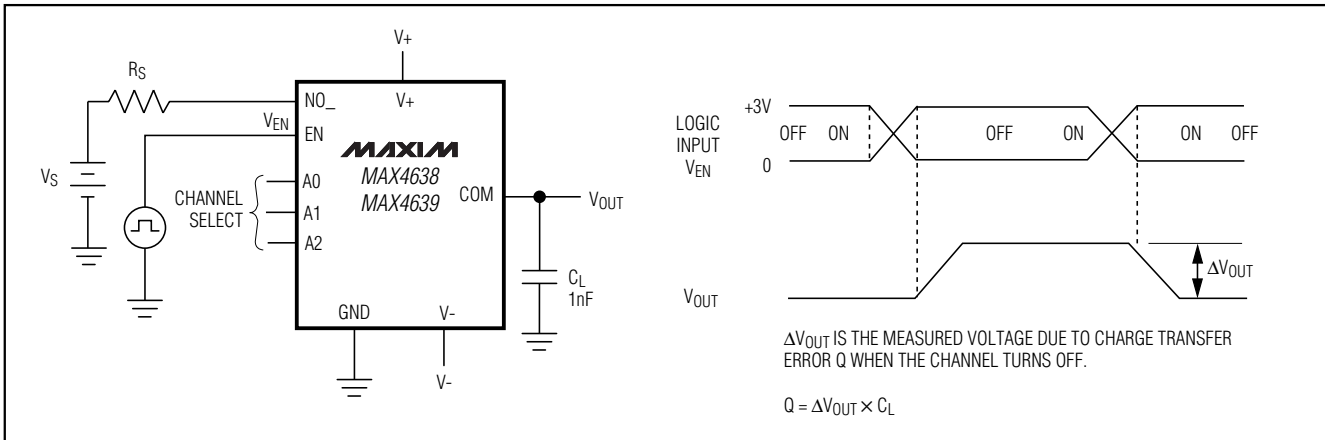
Figure 5. Charge Injection
