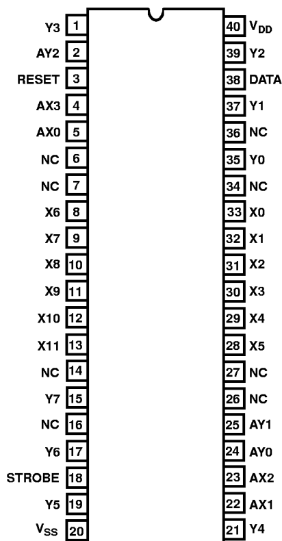
CD22M3493 (PDIP) TOP VIEW
