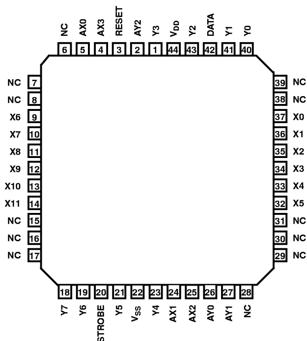
CD22M3493 (PLCC) TOP VIEW
