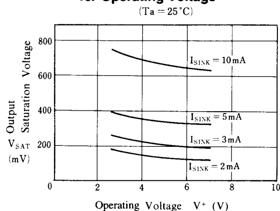
Output Saturation Voltage vs. Operating Voltage
