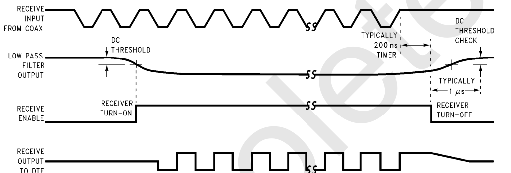
FIGURE 2. Receiver Timing
