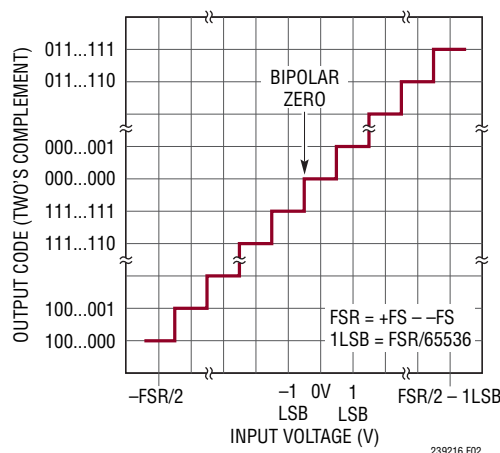
Figure 2. LTC2392-16 Two's Complement Transfer Function
