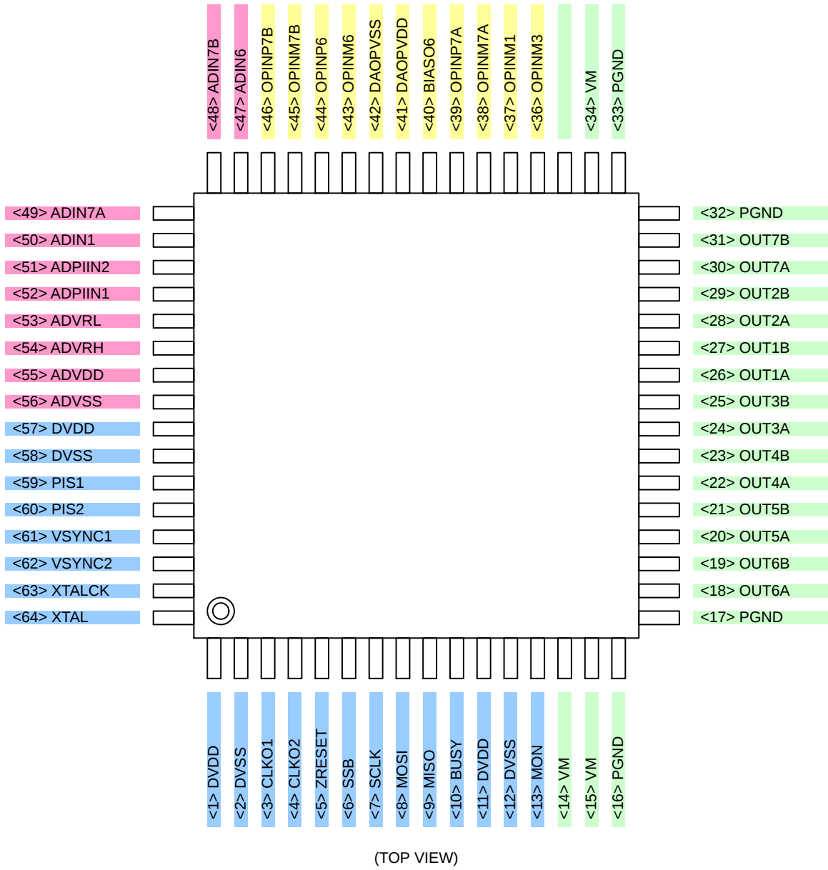
Figure 5. TQFP64 (7x7)
