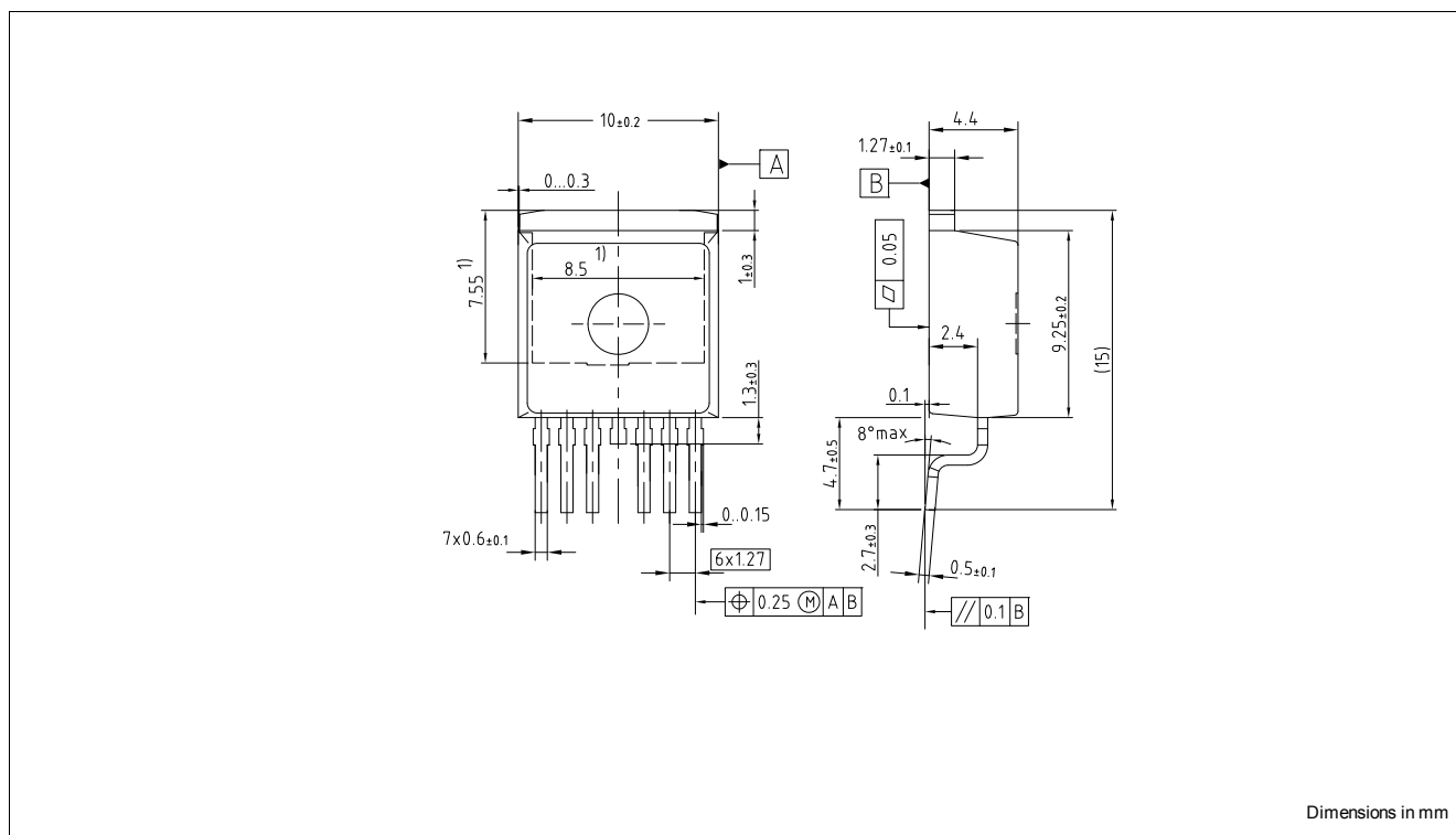
Figure 32 PG-TO-263-7-10 (RoHS-Compliant)
