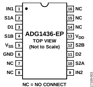
Figure 3. Pin Configuration
