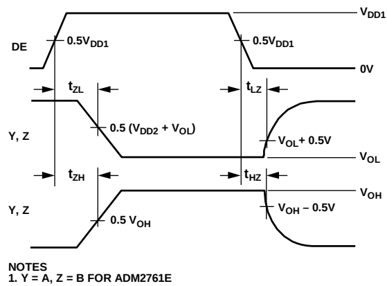
Figure 5. Driver Enable or Disable Timing
