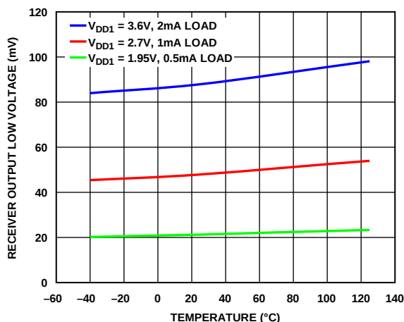
Figure 27. Receiver Output Low Voltage vs. Temperature
