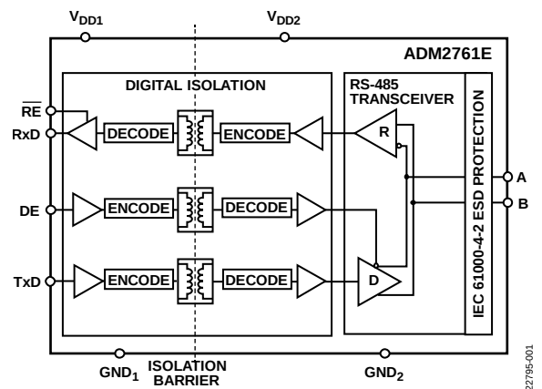
Figure 1. ADM2761E
