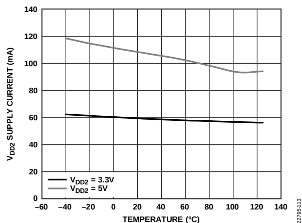
Figure 13. V DD2 Supply Current vs. Temperature, Data Rate = 500 kbps, R L = 54 Ω
