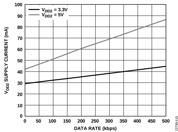
Figure 15. V DD2 Supply Current vs. Data Rate, T A = 25°C, R L = 120 Ω
