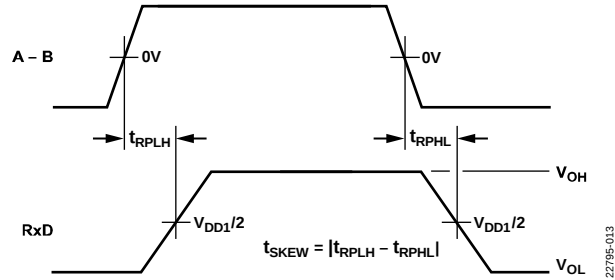
Figure 4. Receiver Propagation Delay
