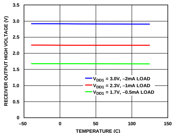
Figure 26. Receiver Output High Voltage vs. Temperature
