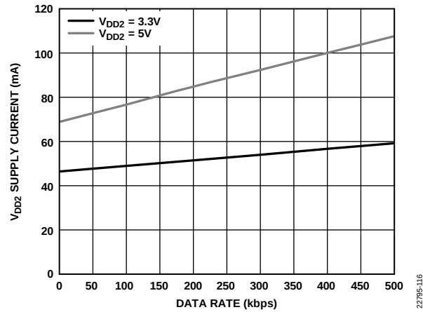
Figure 16. V DD2 Supply Current vs. Data Rate, T A = 25°C, R L = 54 Ω
