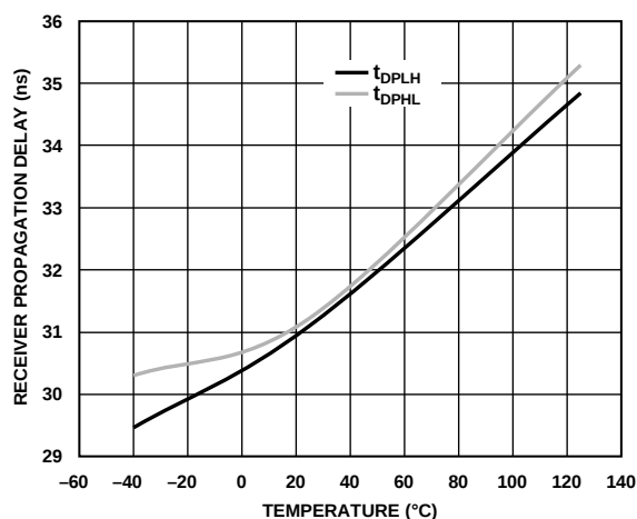
Figure 28. Receiver Propagation Delay vs. Temperature
