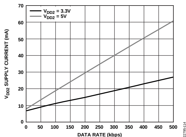
Figure 14. V DD2 Supply Current vs. Data Rate, T A = 25°C, No Load
