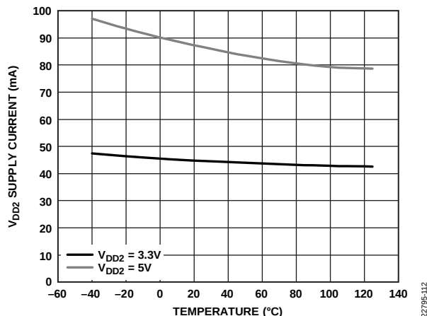
Figure 12. V DD2 Supply Current vs. Temperature, Data Rate = 500 kbps, R L = 120 Ω
