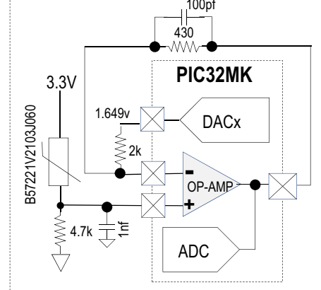
0-100°C NTC Temperature Sensor
