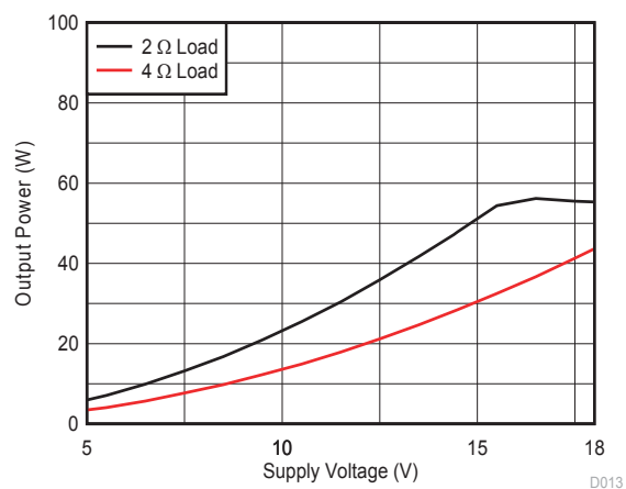
Figure 7-8. Output Power vs Supply Voltage
