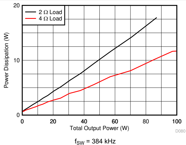
Figure 7-24. Power Dissipation vs Total Output Power
