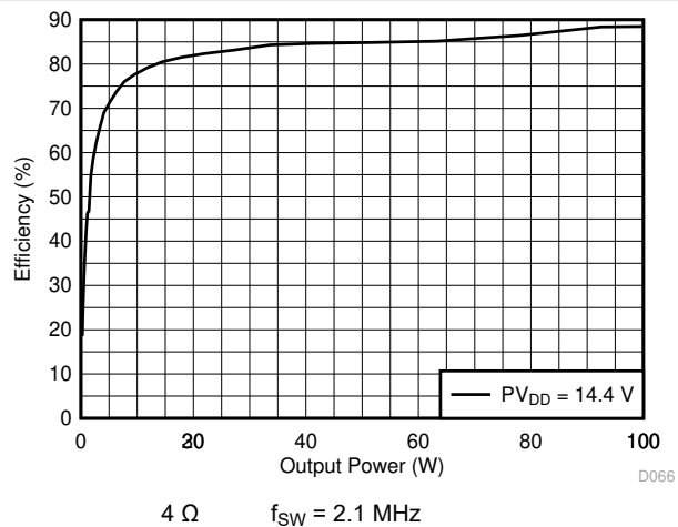
Figure 7-12. PVDD Power Efficiency vs Total Output Power
