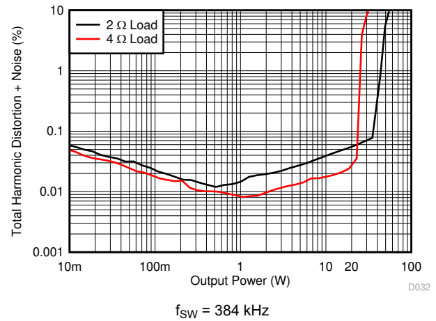
Figure 7-20. PBTL THD+N vs Power
