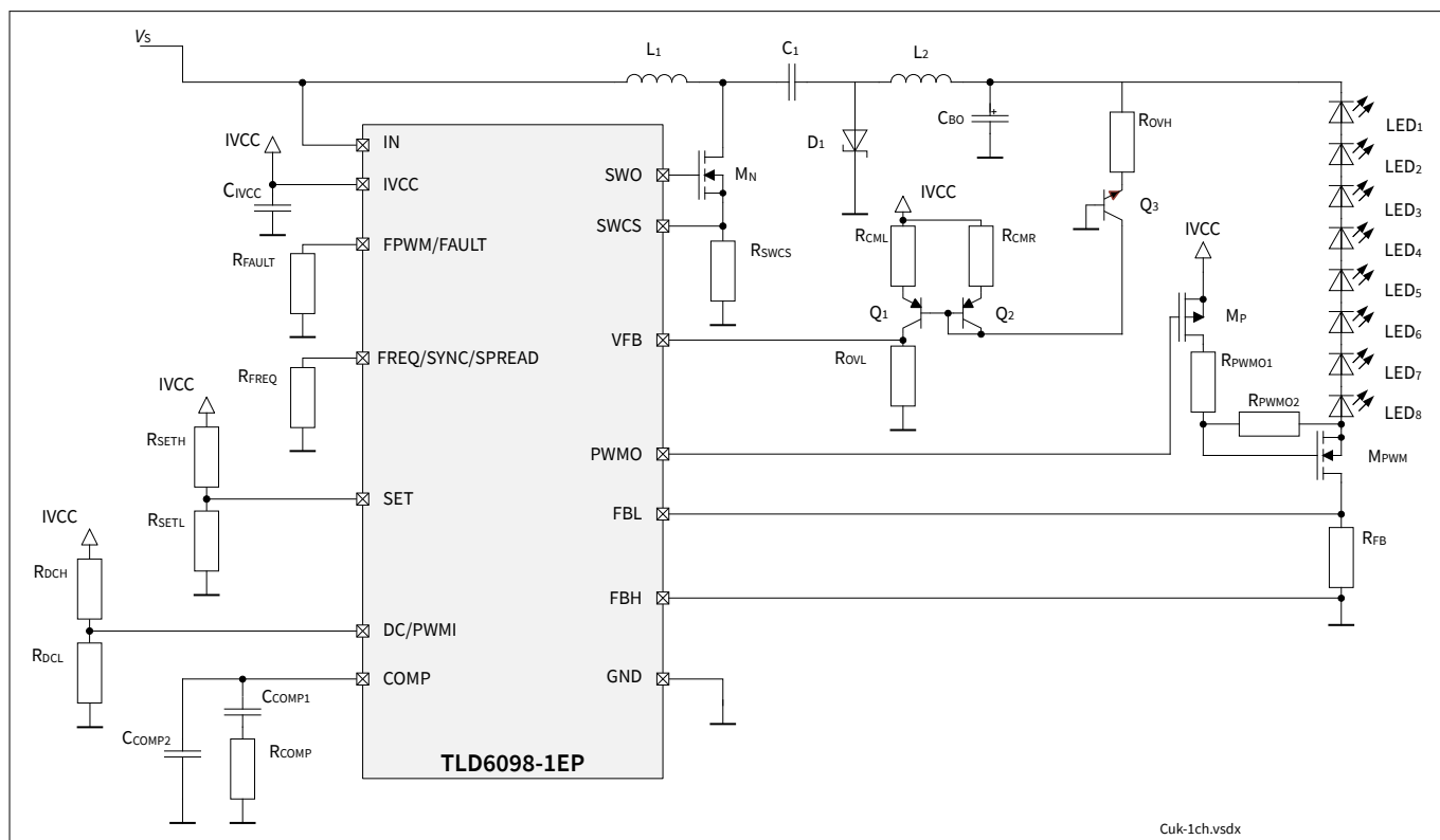
Figure 29 Cuk application schematic
