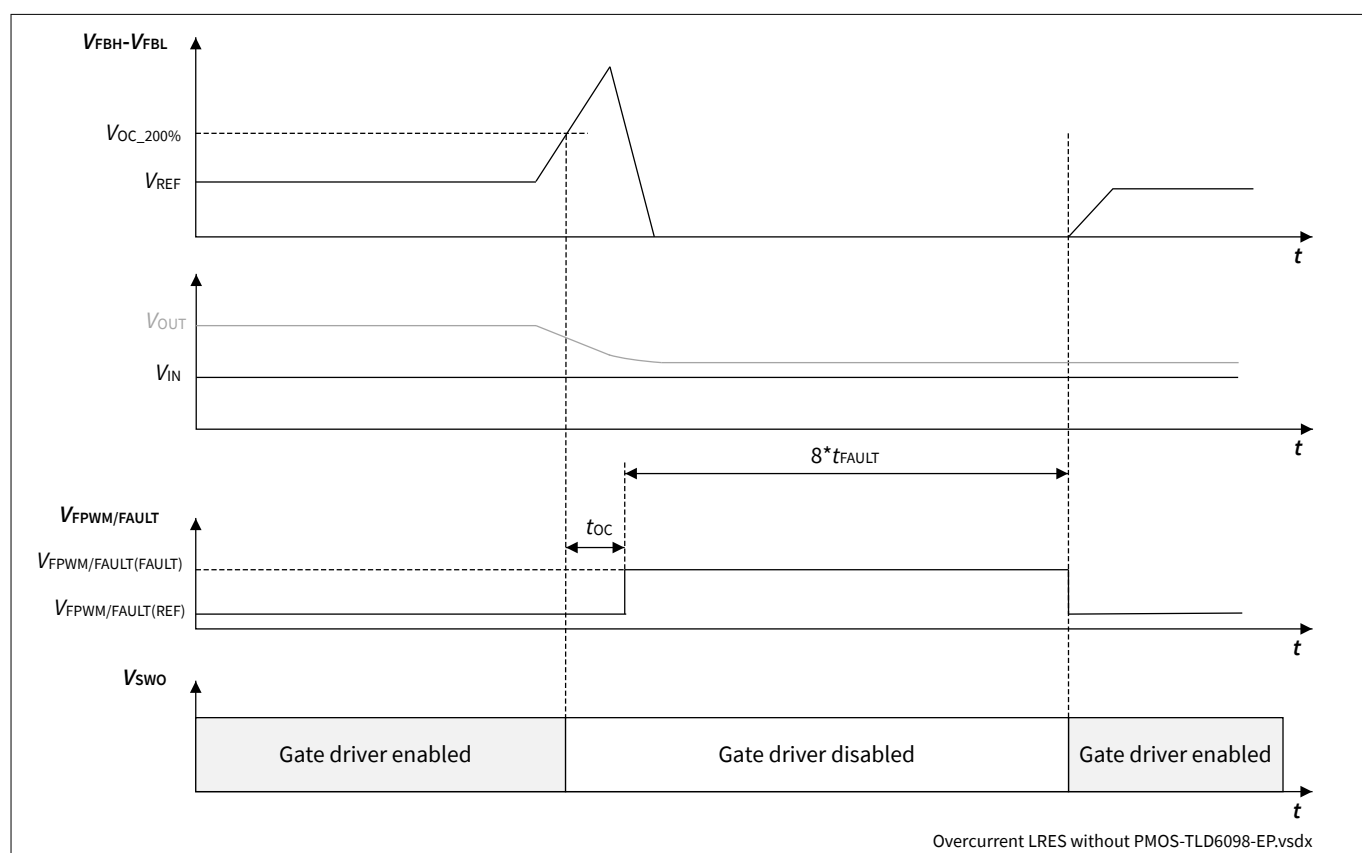
Figure 24 System behavior R_{FPWM/FAULT(L)} during overcurrent detection without PMOS as dimming/protection element
