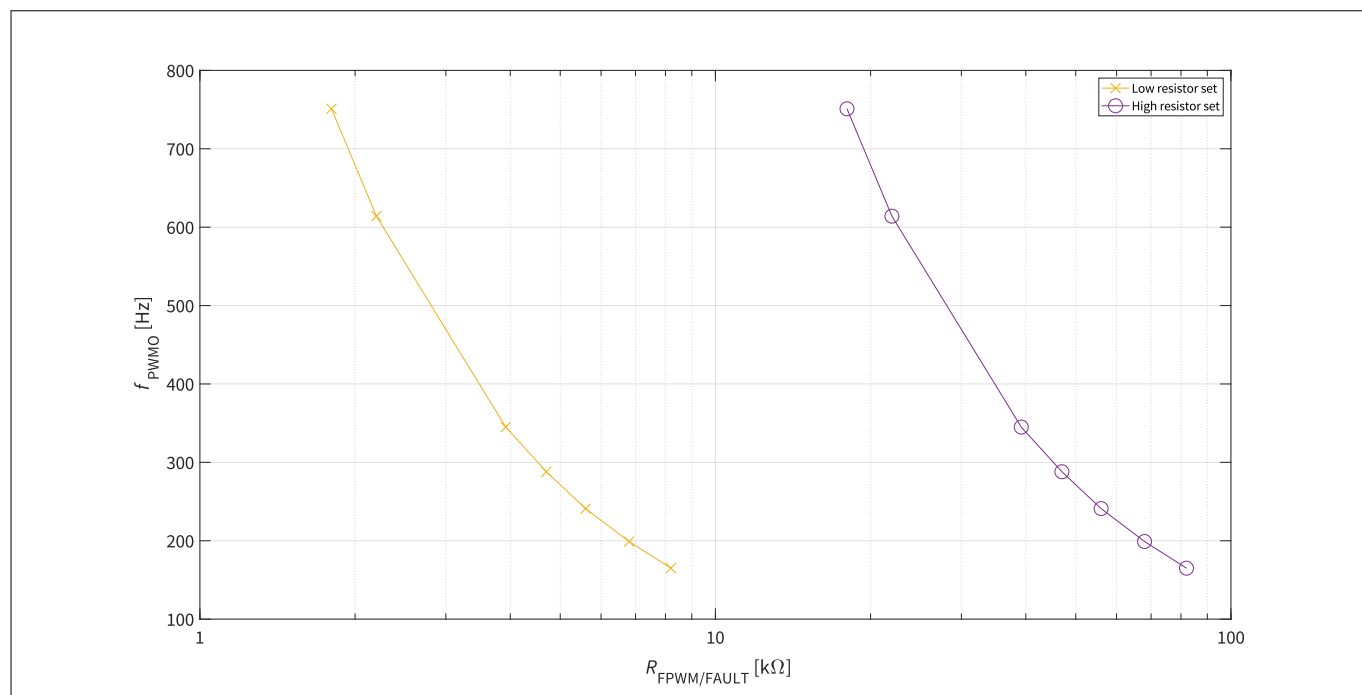
Figure 15 Relationship between R_{FPWM/FAULT} and the frequency of PWM0
