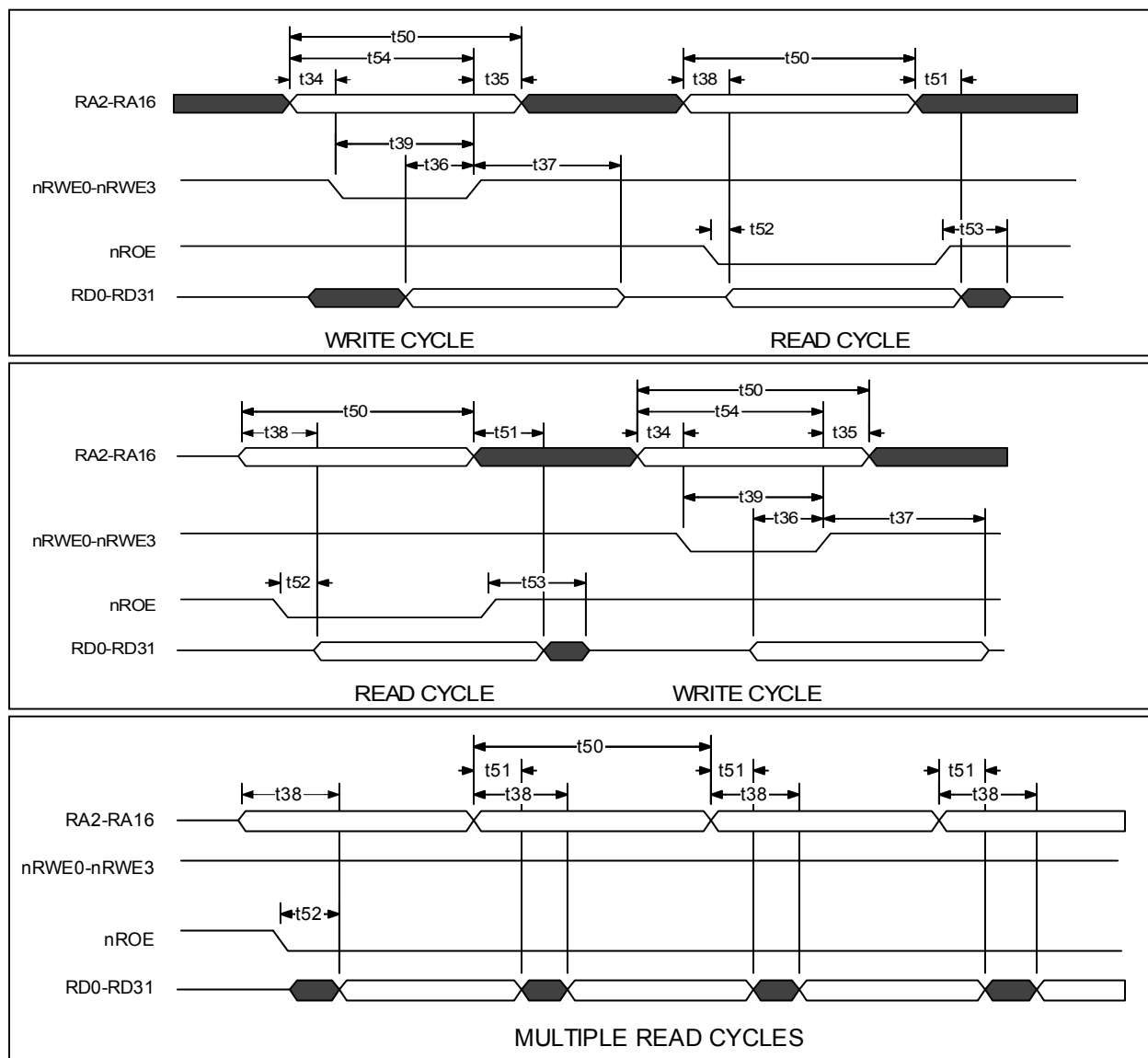
Figure 9.9 - SRAM Interface
