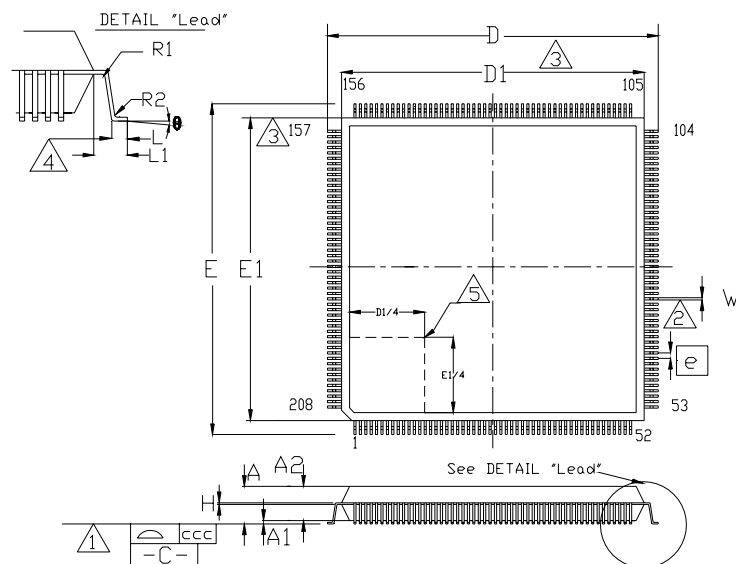
Figure 10.1 - 208 Pin QFP Package Outline
