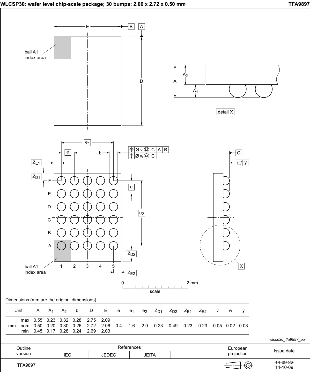
Fig 5. Package outline TFA9897 (WLCSP30)
