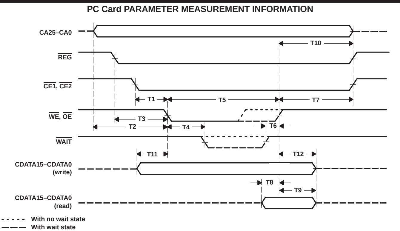
Figure 24. PC Card Memory Cycle
