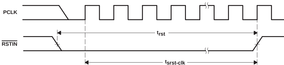
Figure 22. \overline{\text{RSTIN}} Timing Waveforms
