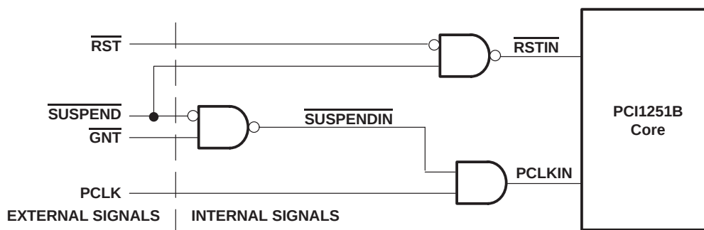
Figure 14. SUSPEND Functional Implementation
