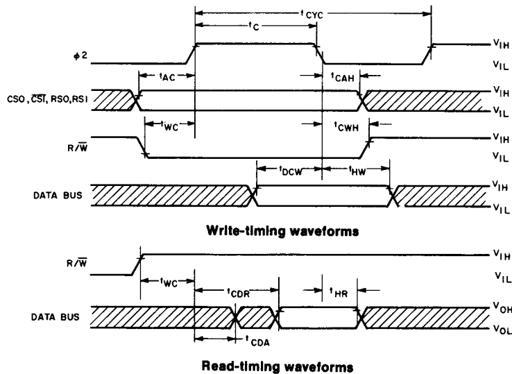
Fig. 22 - Timing waveforms.
