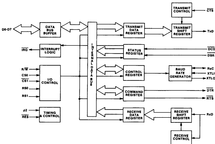
Fig. 2 - Internal organization.
