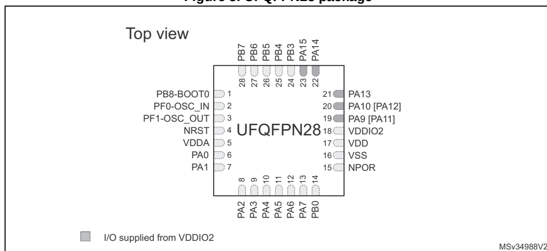
Figure 5. UFQFPN28 package
