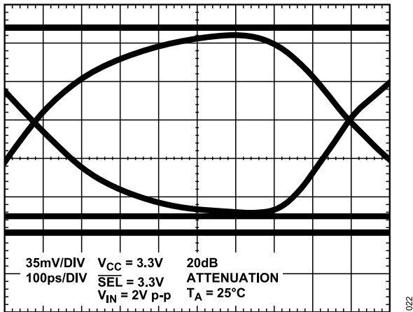
Figure 22. Eye Pattern; 1.244 Gbps, V_{CC} = 3.3 V , PRBS 31
