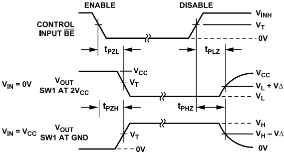
Figure 27. Enable and Disable Time
