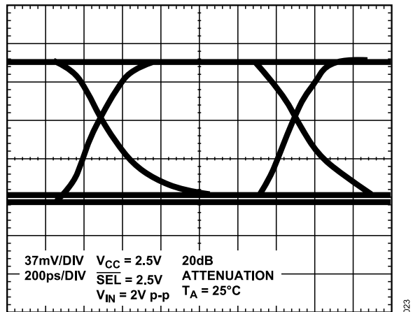
Figure 23. Eye Pattern; 1 Gbps, V_{CC} = 2.5 V , PRBS 31
