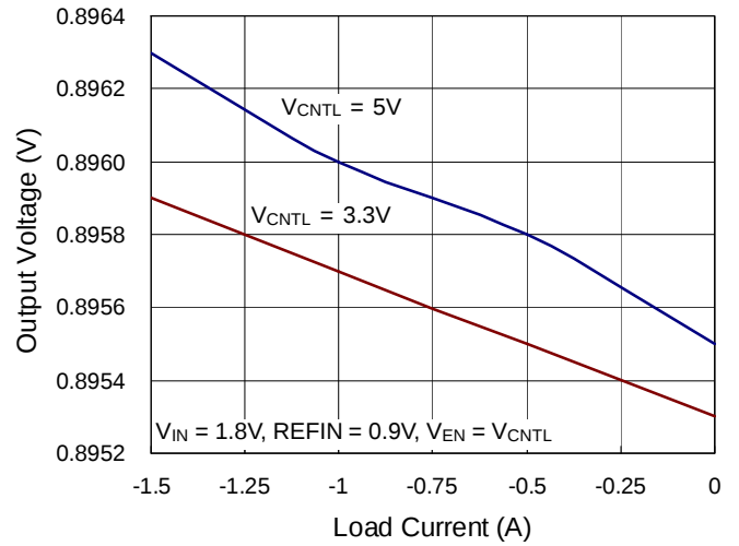
DDR2 Output Voltage vs. Load Current
