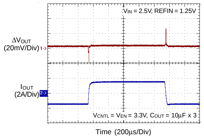
1.25V OUT @ \pm 1.5A Transient Response
