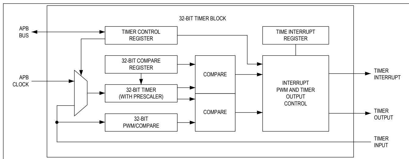
Figure 9. 32-Bit Timer
