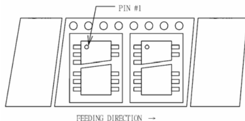
14 Pin SOP Package
