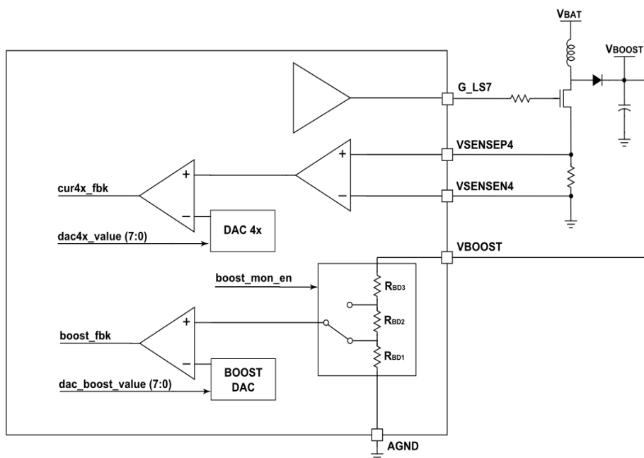
Figure 11. Boost Converter Topology for Fixed Frequency Mode
