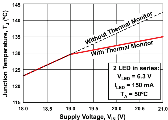
Figure 12: Junction Temperature versus Supply Voltage
