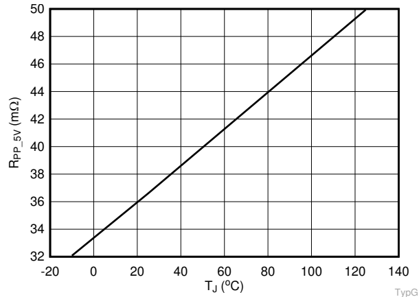
Figure 7-1. PP_5V Rdson vs. Temperature.
