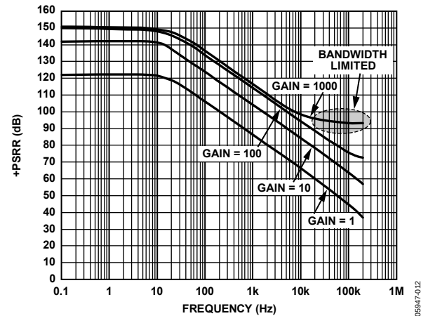
Figure 13. Positive PSRR vs. Frequency, RTI ( G = 1 to 1000)
