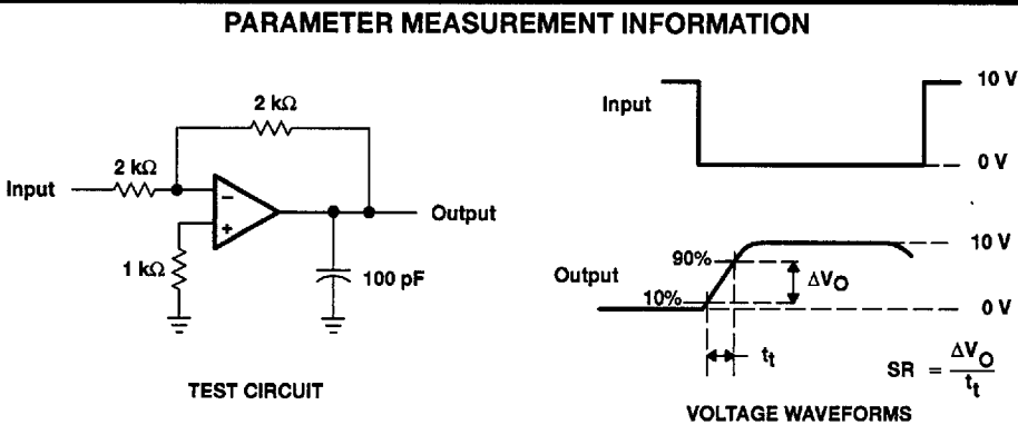
Figure 1. Slew Rate
