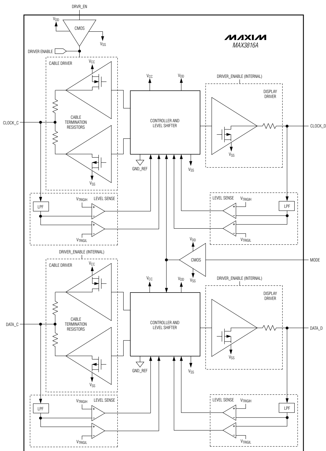
Figure 2. Functional Diagram
