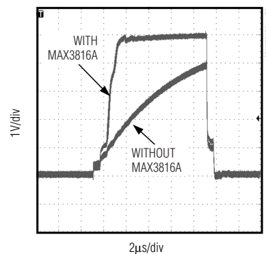
DATA_C TRANSIENT RESPONSE WITH AND WITHOUT MAX3816A, 60m CABLE LOAD (4700pF)
