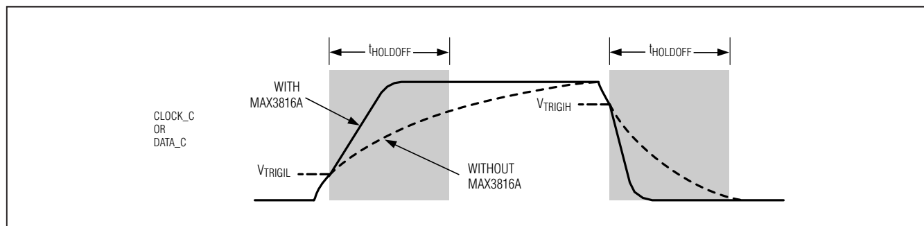
Figure 3. Holdoff Operation
