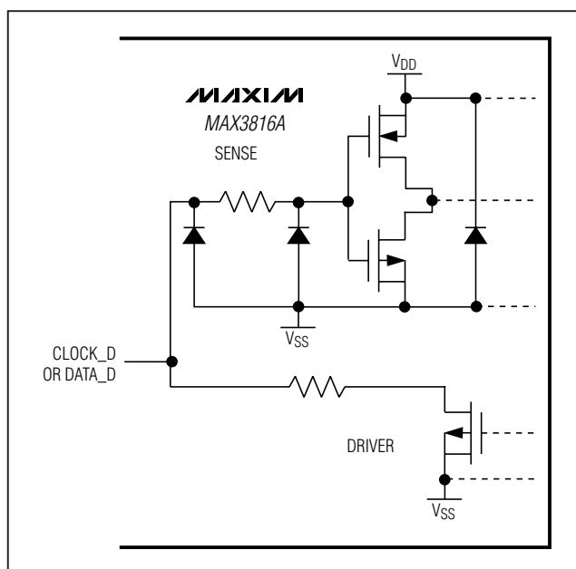
Figure 10. CLOCK_D/DATA_D Equivalent Interface Structure
