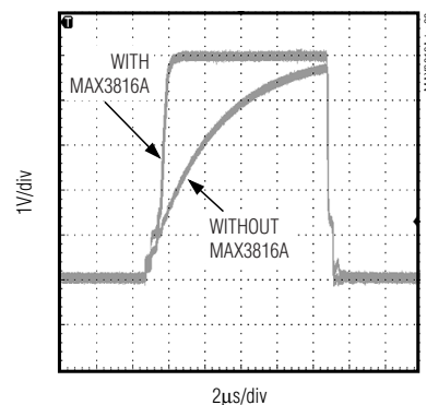
CLOCK_C TRANSIENT RESPONSE WITH AND WITHOUT MAX3816A, 30m CABLE LOAD (2350pF)
