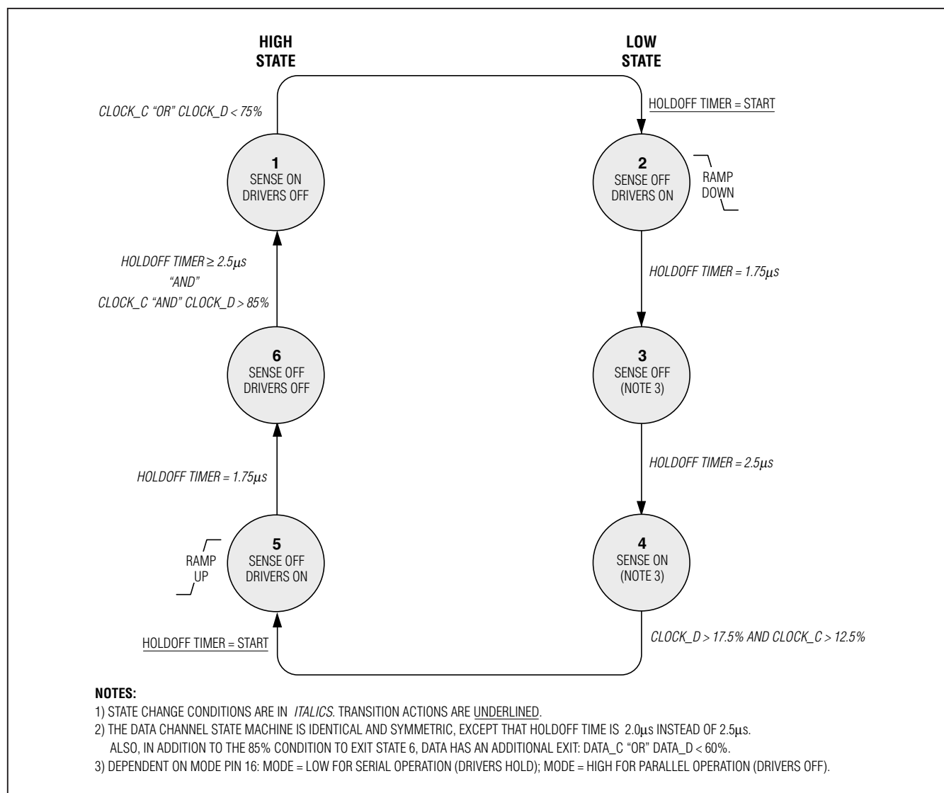
Figure 1a. Clock State Machine Diagram
